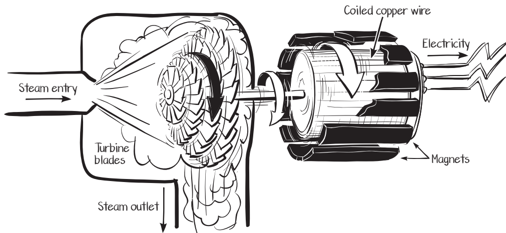
Turbine Generator
