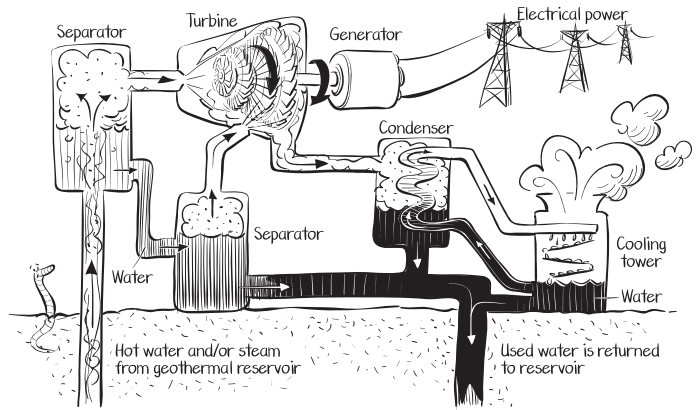
Flash Power Plant
