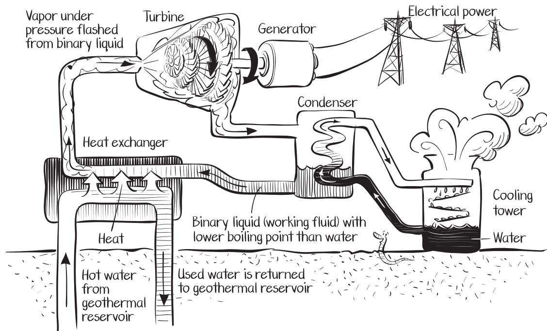
Binary Power Plant
