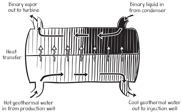
Binary Power Plant Heat Exchanger
