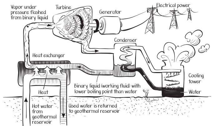
Binary Power Plant
