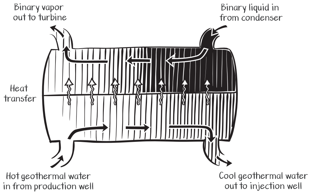
Binary Power Plant Heat Exchanger
