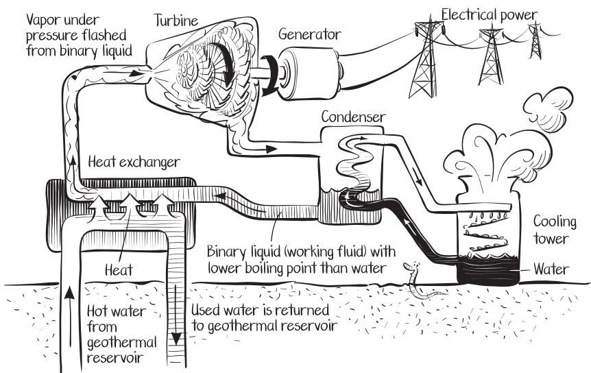
Binary power plant
