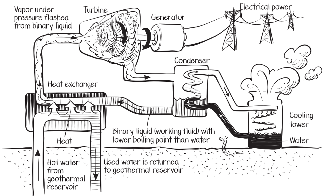
Binary Power Plant
