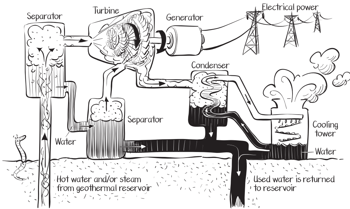
Flash Power Plant
